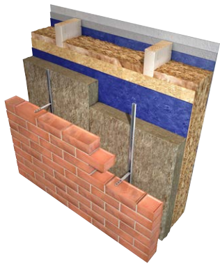
Timber frame - single layer
