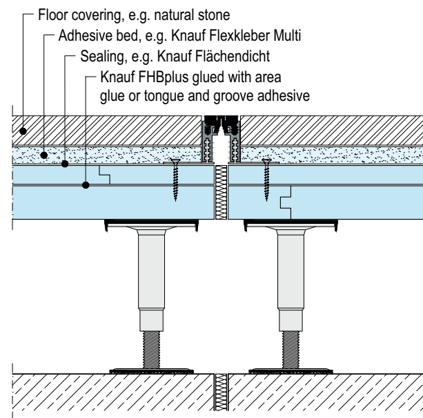
F182.de-V10 GIFAfloor FHBplus 32+18 Joint with fire resistance underlay
