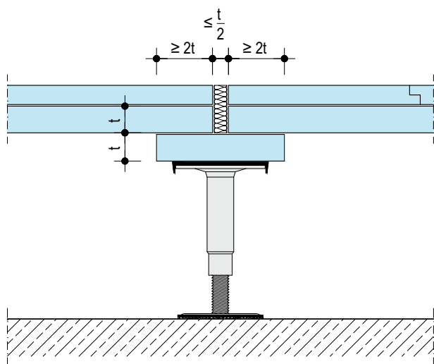
F182.de-V11 GIFAfloor FHBplus 25+18 access opening / transition to hollow floor panels
