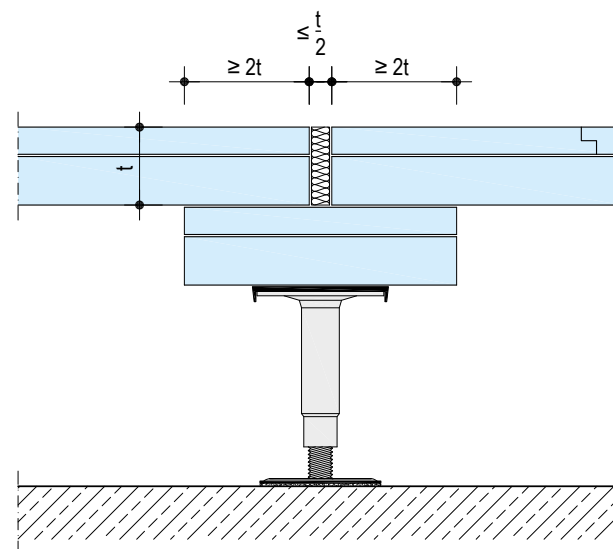
F182.de-V11 GIFAfloor FHBplus 25+18 access opening / transition to hollow floor panels
