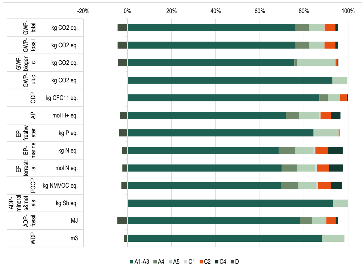
Contribution to environmental impact per each module for 1 m 2 of installed Knauf RED 15mm gypsum plasterboard
