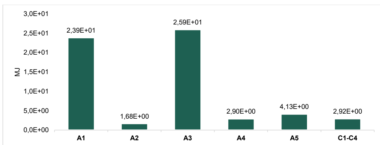
Primary energy demand per 1 m 2 of installed Knauf RED 15mm gypsum plasterboard
