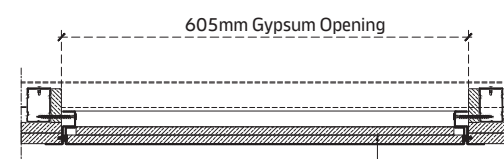
SECTION A
