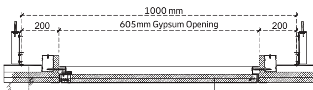
SECTION A
