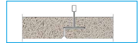
RAND D (VK-10) (alleen T35)
