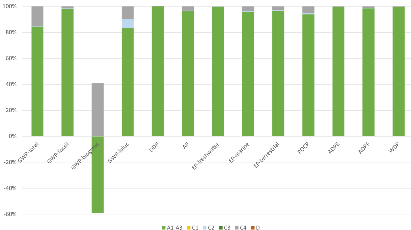
Hot-spot analysis of the KCS mineral ceiling tiles - Adagio Acoustic+ (19 mm)
