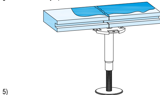
5) Apply glue to full surface.
