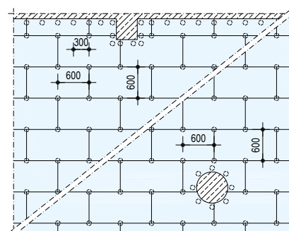
Pedestal arrangement, e.g. with rising components
