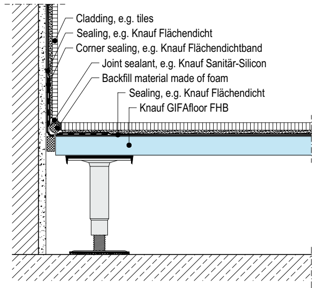
F181.de-V2 Connection to solid wall
