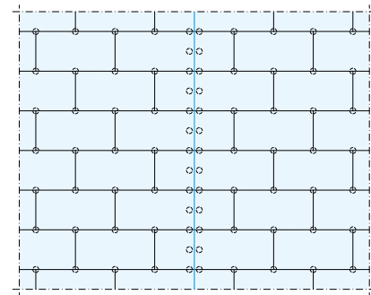
Configuration of a control joint with half the pedestal spacing in the perimeter area (shown with double row of pedestals).
