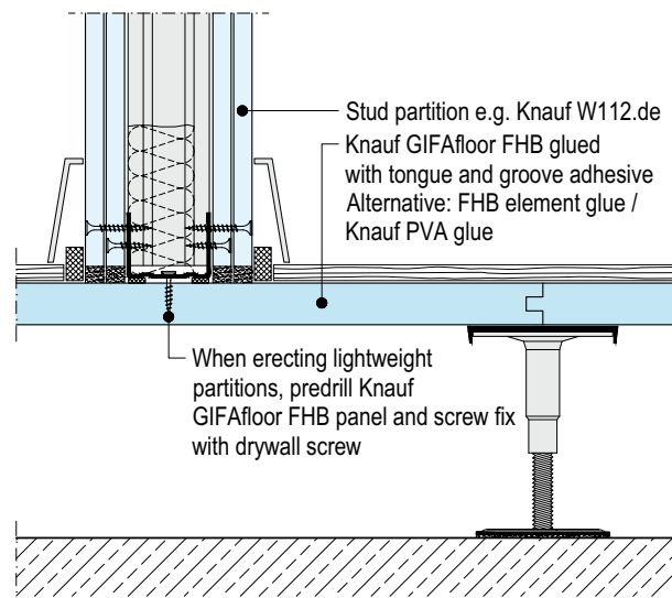
F181.de-V8 Partition on GIFAfloor FHB – W112.de
