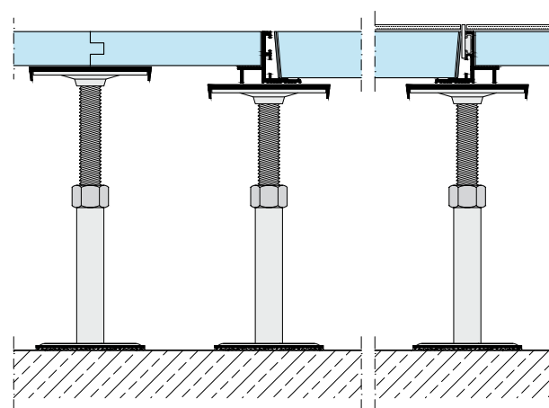
F181.de-V13 Installation revision frame / transition profile
