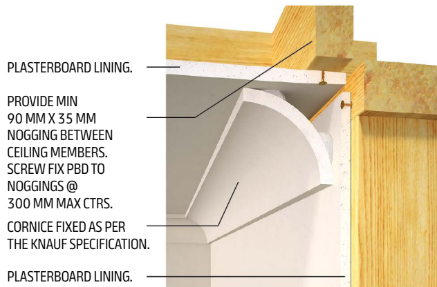
Figure 41: Cornice Detail
