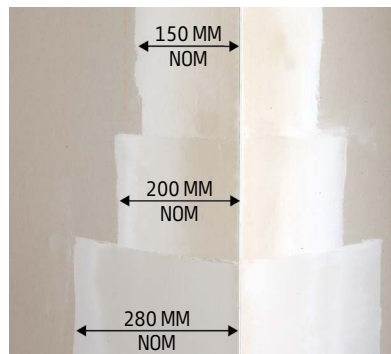
5. External corner jointing system
