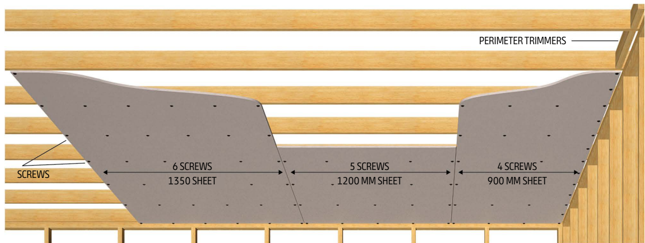
Figure 22: Screw Fixing (only) Layout for Ceilings
