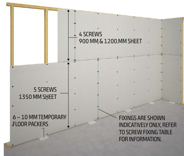
Figure 31: Screw Fixing to Walls
