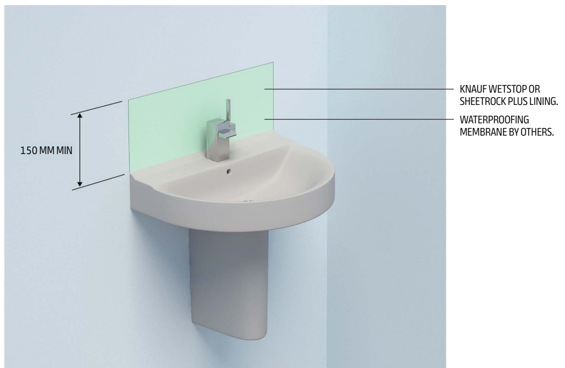
Figure 57: Waterproofing of Basin
