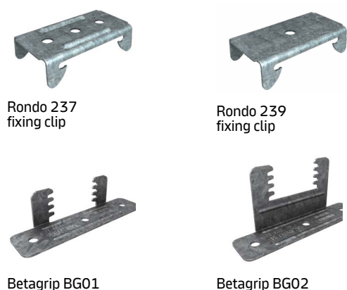
Figure 47: Masonry Fixing Clips
