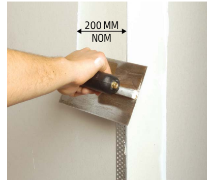
3. Apply second coat to corner faces
