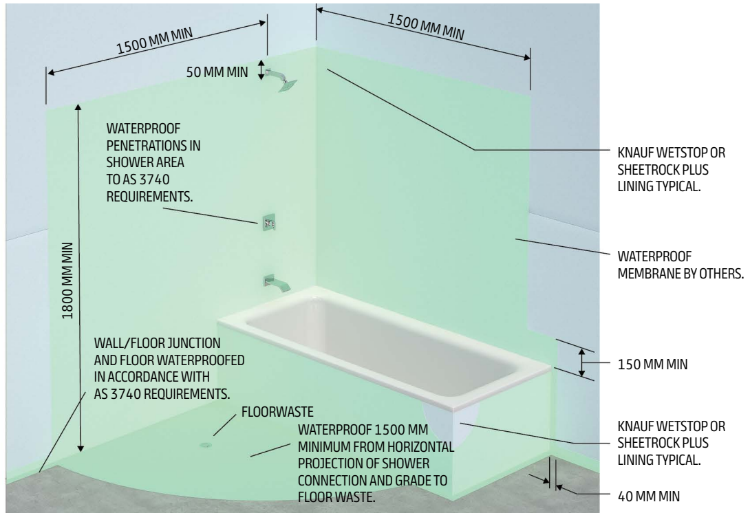
Figure 54: Waterproofing of Unenclosed Shower Over Bath
