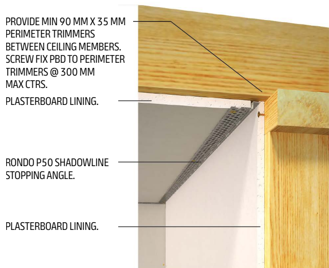
Figure 44: Shadowline Angle 2
