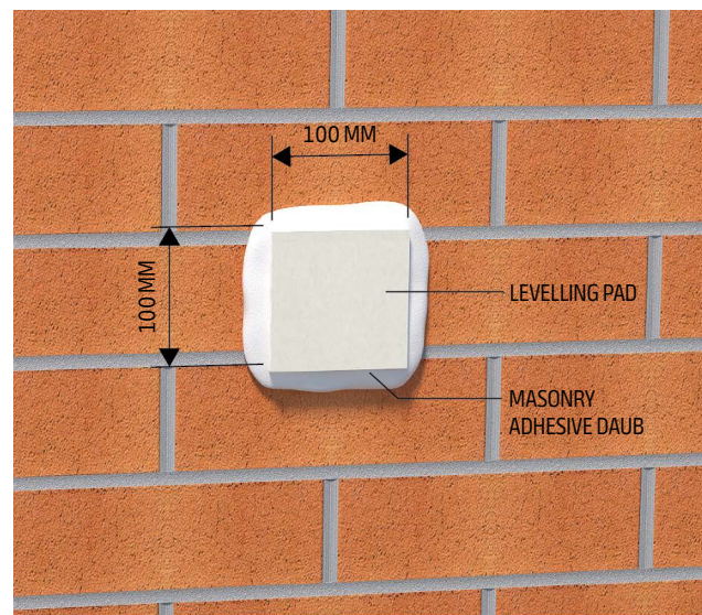
Figure 46: Levelling Pads
