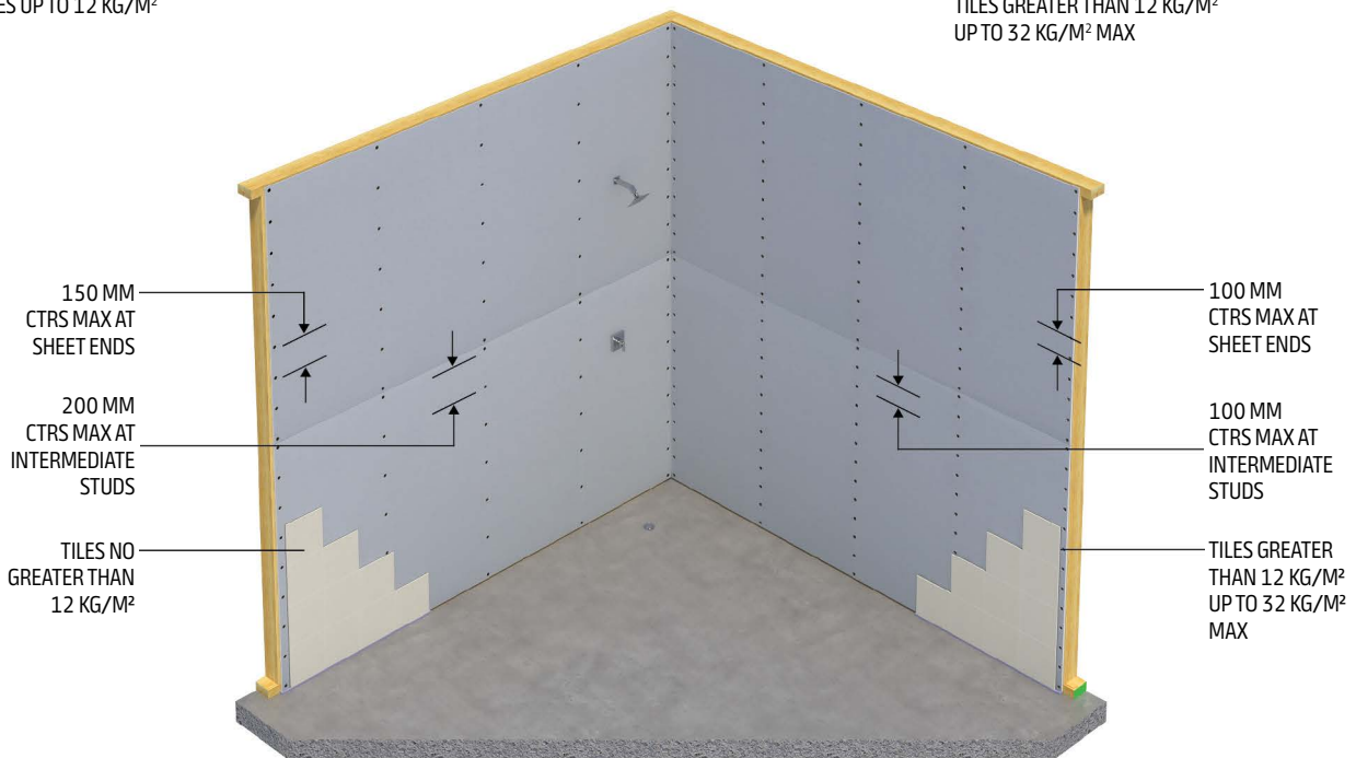
Figure 51: Plasterboard Fixing in Tiled Areas
