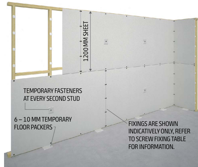
Figure 30: Combination Adhesive and Screw Fixing on Walls
