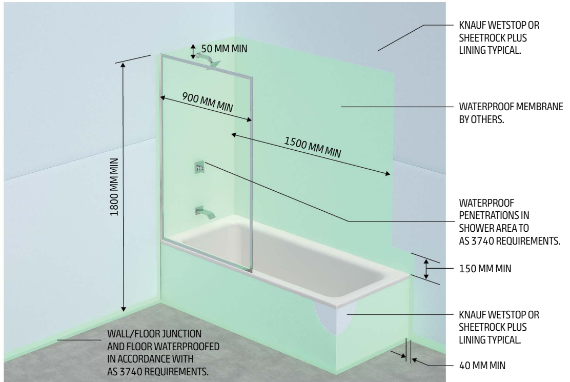
Figure 52: Waterproofing of Enclosed Shower Over Bath
