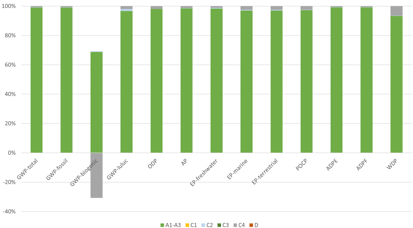
Hot-spot analysis of the KCS stone wool panels - TOPIQ Efficient pro (Board) (20 mm)
