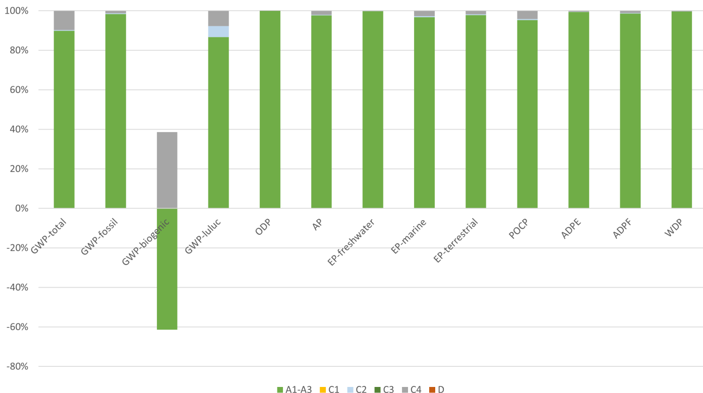
Hot-spot analysis of the KCS mineral ceiling tiles - Adagio HD+ (19 mm)
