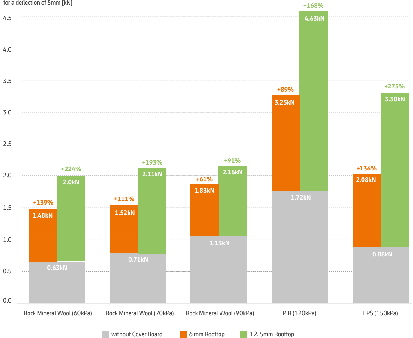
Point Load for a deflection of 5mm [kN]
