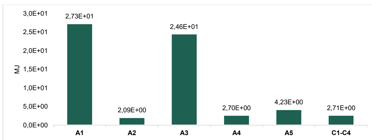
Primary energy demand per 1 m 2 of installed Knauf Blue 12.5mm gypsum plasterboard
