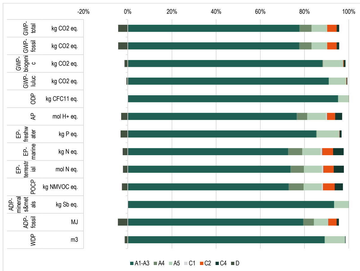
Contribution to environmental impact per each module for 1 m 2 of installed Knauf Blue 12.5mm gypsum plasterboard
