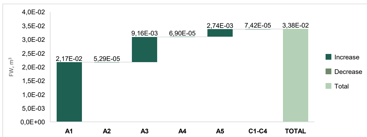
Net freshwater use for 1 m 2 of installed Knauf Blue 12.5mm gypsum plasterboard
