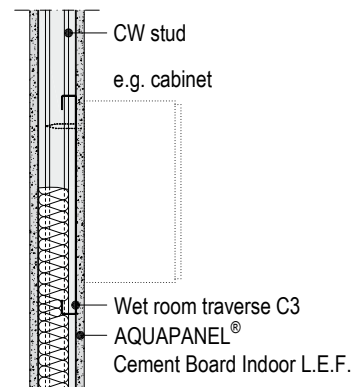
W234.de-V17 Vertical section – Design with CW stud
