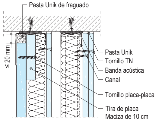
W634.es-B1 Junta vertical
