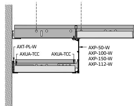
Downstand margin with AXONIS Profile
