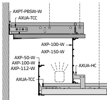
Concealed lighting detail with plasterboard margin and AXONIS Profile
