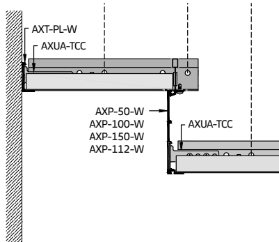
Upstand margin with AXONIS Profile
