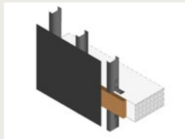
3. Insulate floor front and temporarily bond water barrier to the studs
