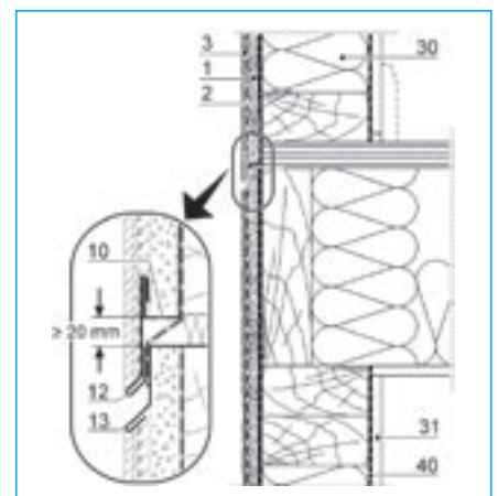
Horizontal expansion joint (formation in the area of ceilings)
