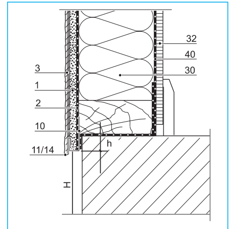
Base formation
