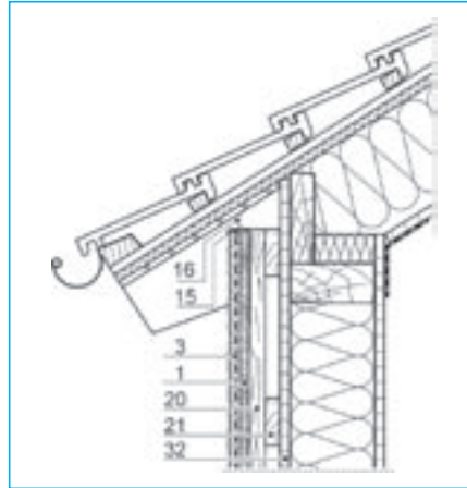
Eave formation
