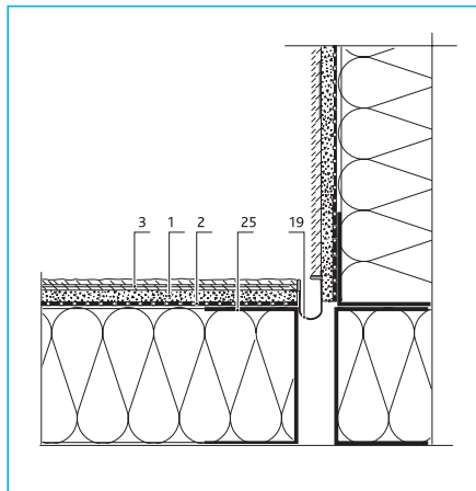
Internal corner
