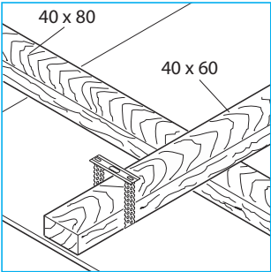
Direct securing with only one batten
