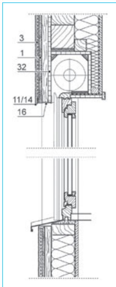
Upper and lower window join
