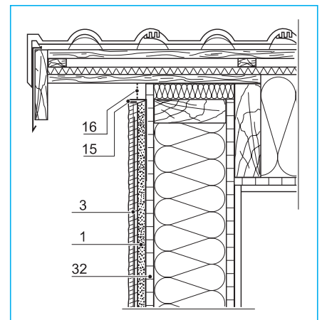
Verge formation
