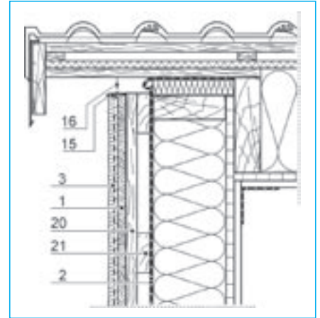
Verge formation
