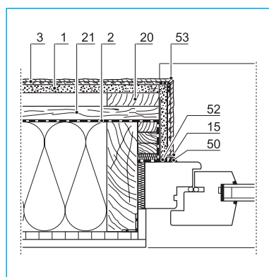
Side window join
