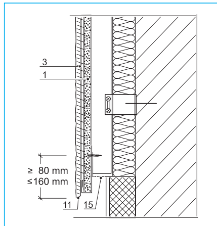
Base formation
