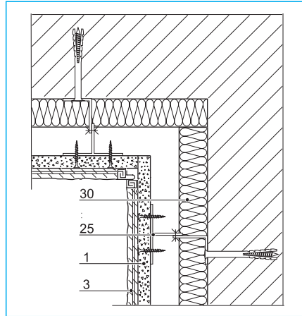
Internal corner
