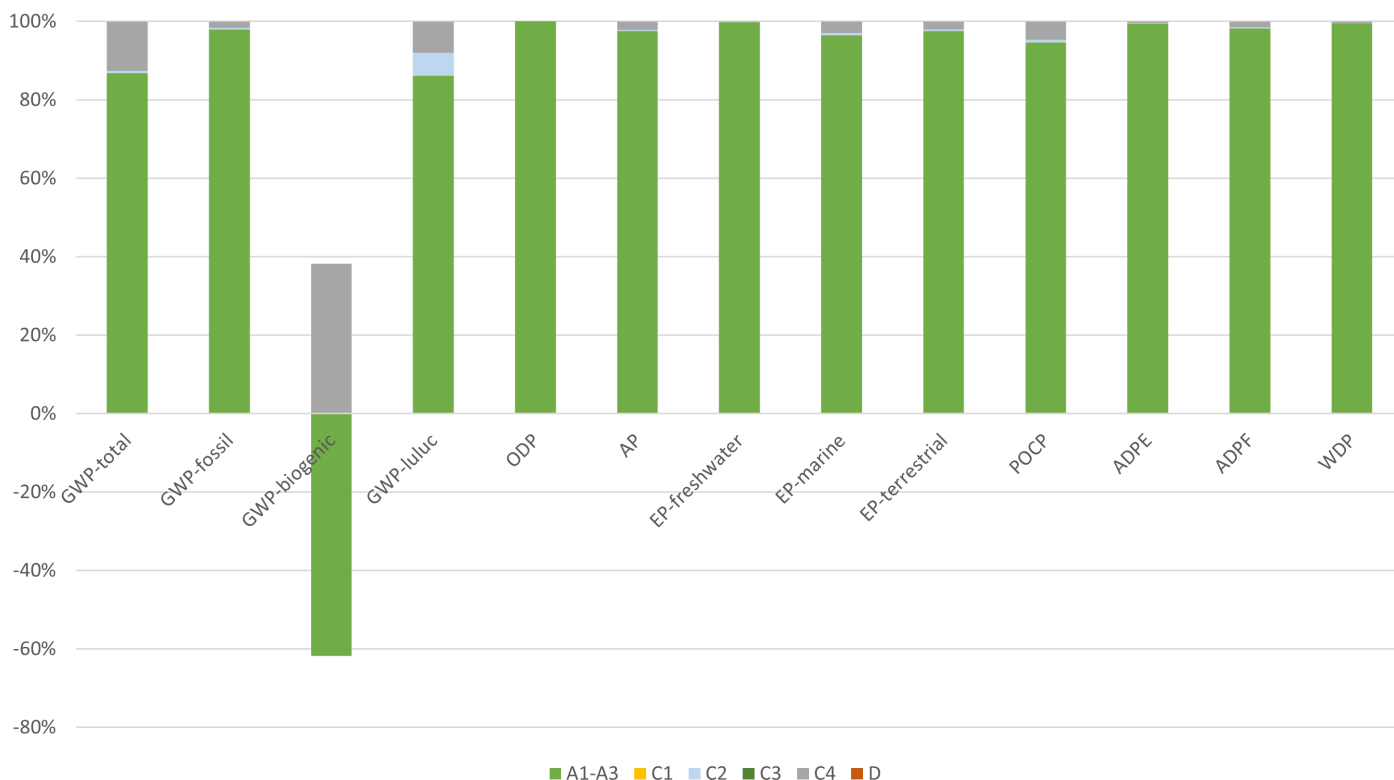
Hot-spot analysis of the KCS mineral ceiling tiles - Adagio HD+ (30 mm)
