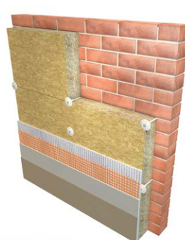
External Wall Insulation
