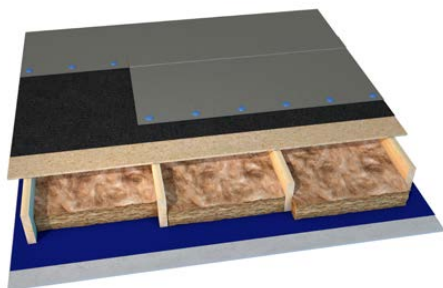
Flat Roof - Cold Roof
