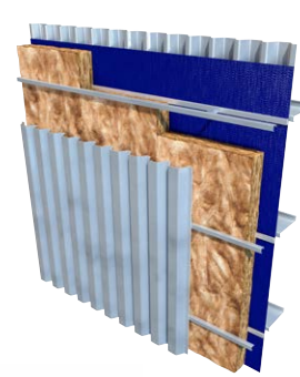
Built-Up Metal Wall
