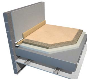
Separating Concrete Floor
