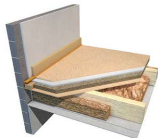
Separating Timber Floor Upgrade to an existing timber floor with new platform floor
