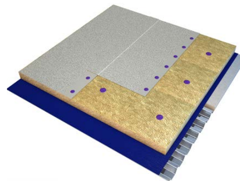
Flat Roof - Warm Roof
