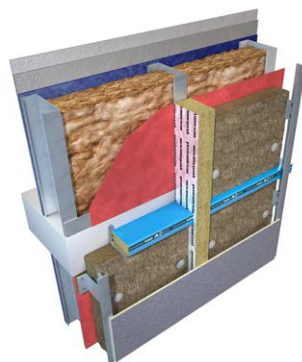
Cavity Barriers
