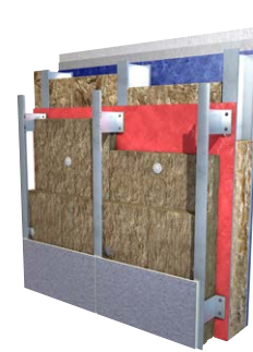
Rainscreen Façade System
