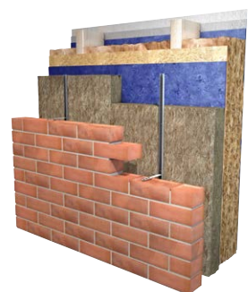
Frame Construction with Masonry Outer
