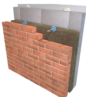
External Masonry Cavity Walls - Partially Filled
