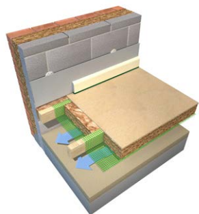
Suspended Timber Ground Floor
