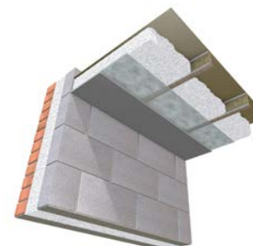
Insulated Floor above Integral Garage
