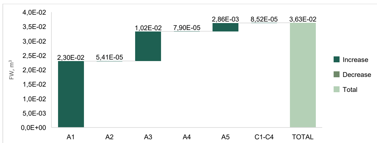
Net freshwater use for 1 m 2 of installed Knauf Blue 15mm gypsum plasterboard
