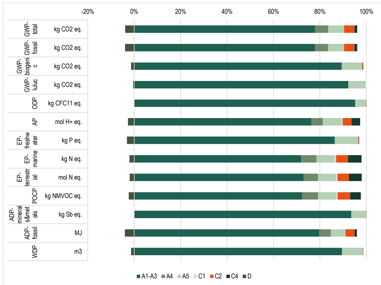
Contribution to environmental impact per each module for 1 m 2 of installed Knauf Blue 15mm gypsum plasterboard
