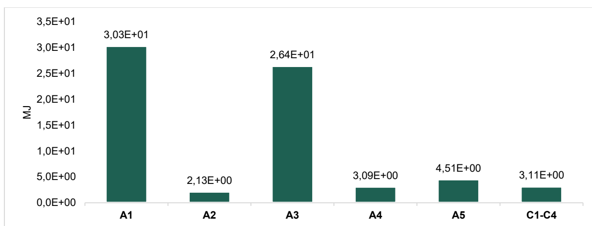
Primary energy demand per 1 m 2 of installed Knauf Blue 15mm gypsum plasterboard
