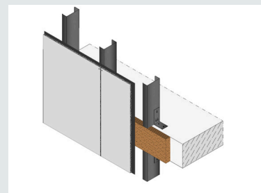
4. Installation de la AQUAPANEL® Cement Board Outdoor
